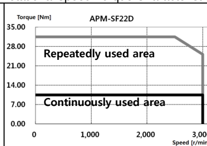
◆ Rotational speed-Torque Characteristics ◆
