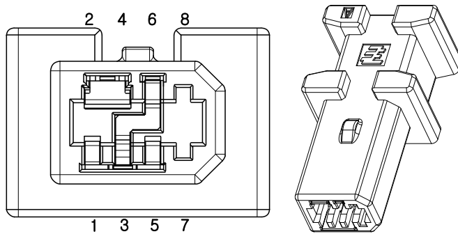
1971153-1(Tyco Electronics)
