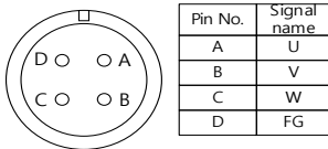
<Power Connector>
