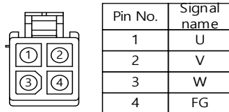
<Power Connector>
