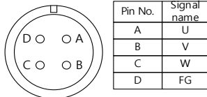
<Power Connector>
