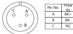
<Brake Connector>
