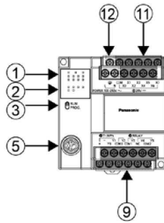
■ L40/L60 Control unit
