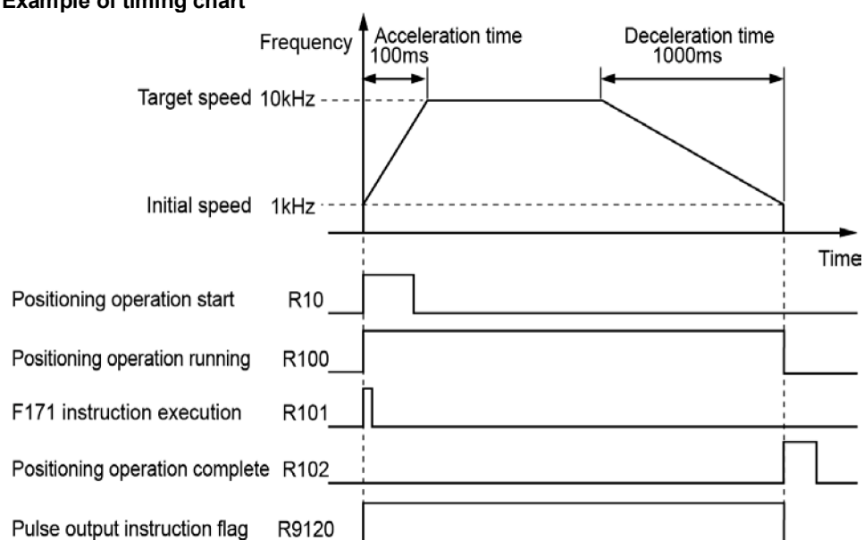
Example of timing chart
